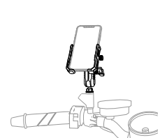
Bolt Head Adapter with 1" Ball Installation (Rearview Mirror disassemble)
